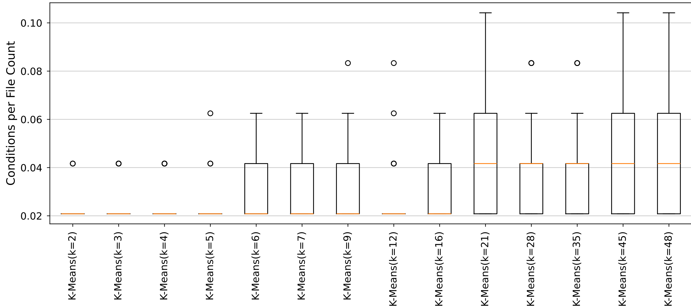
YARA Rules Conditions per File Count Distribution (Cluster4_Size48 dataset)
